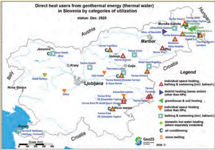
Figure 2: Main categories of direct heat use of geothermal energy from thermal water in Slovenia in 2025 at 30 locations; the Tešanovci greenhouse is considered a separate user, while the district heating system at Benedikt is included as a special case (without thermal water use).
