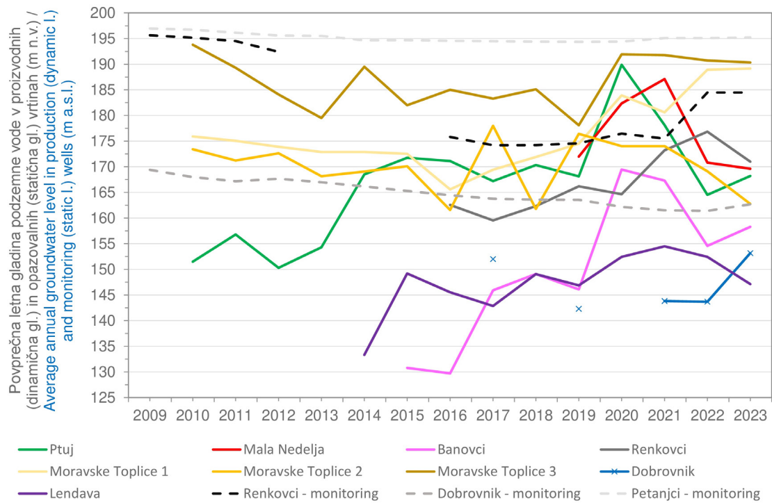
Trend letnih gladin v geotermalnih vrtnah v SV Sloveniji od 2009 do 2023 (vir: GeoZS, ARSO) Trend of yearly groundwater levels in geothermal wells in NE Slovenia from 2009 to 2023 (source: GeoZS, ARSO)
